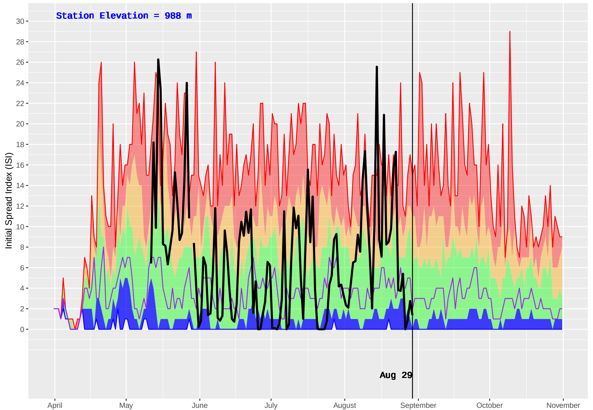
NOEL (437) : Historical (1993–2016) and Current (2018) Daily Initial Spread Index (ISI)
